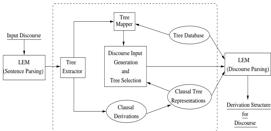
Figure 4. D-LTAG: System Description
