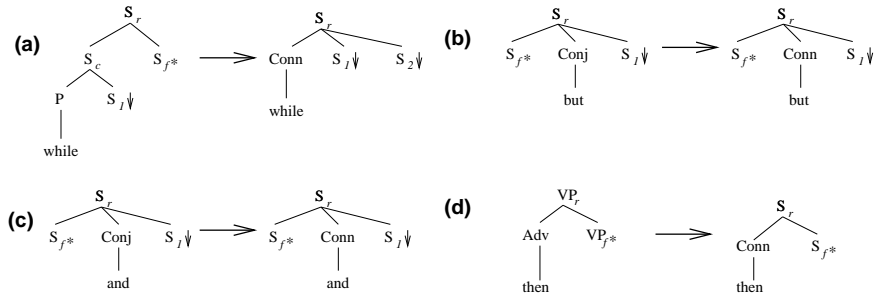
Figure 7. Elementary Tree Mappings for Connectives in Discourse (4)
