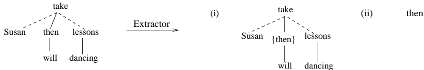
Figure 6. Result of Tree Extractor Applied to Derivation of Susan will then take dancing lessons
