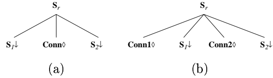
Figure 1. Initial Trees in D-LTAG
