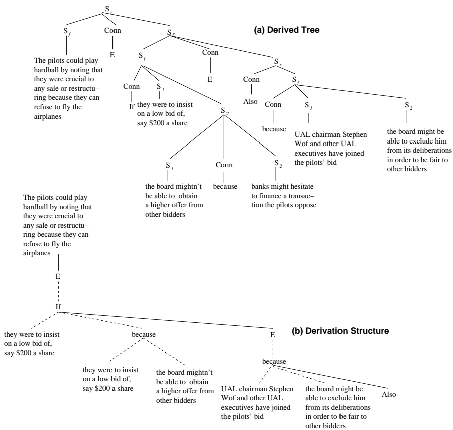
Figure 9. (a) Derived Tree and (b) Derivation Structure for WSJ Discourse in (6)
