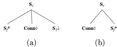
Figure 3. Auxiliary Trees in D-LTAG
