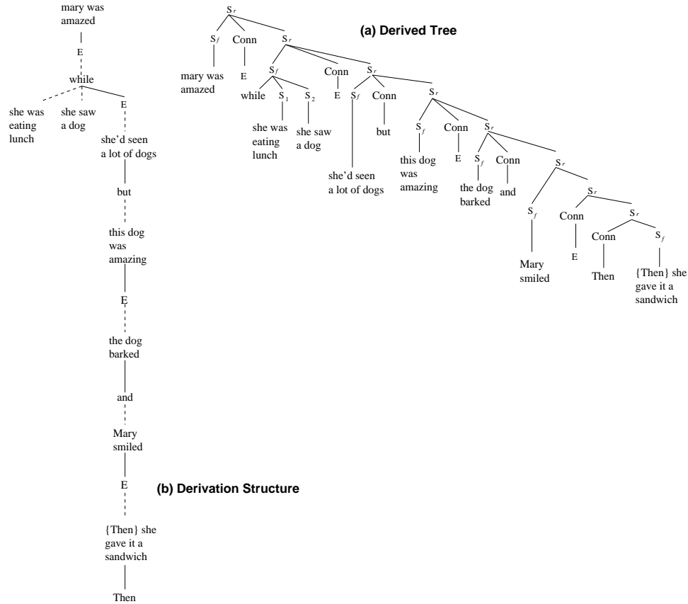
Figure 8. (a) Derived Tree and (b) Derivation Structure for Example Discourse in (4)
